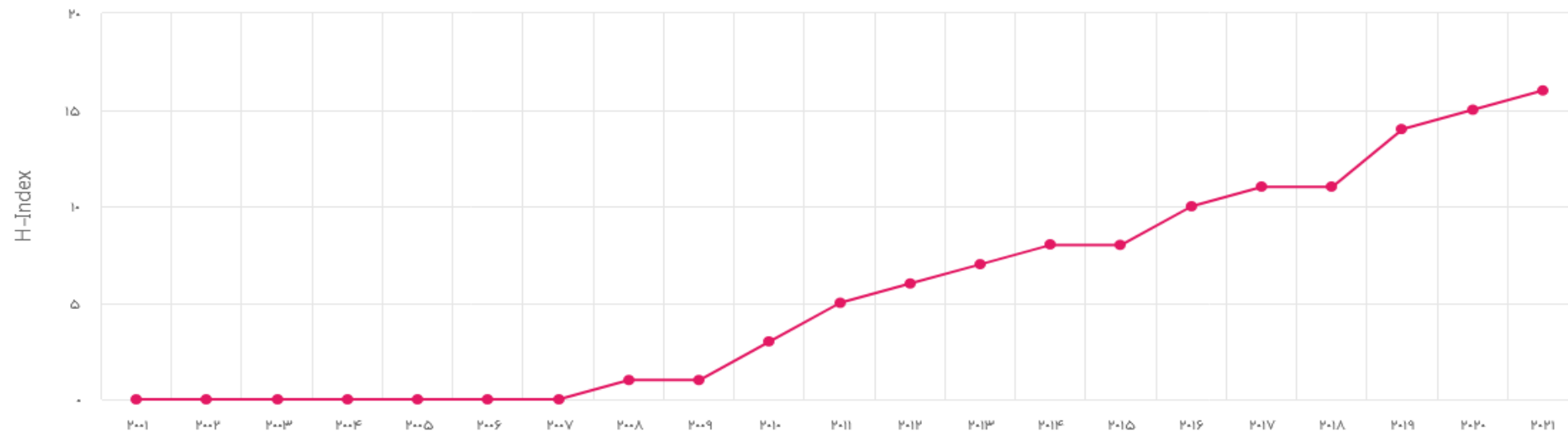
H-Index
